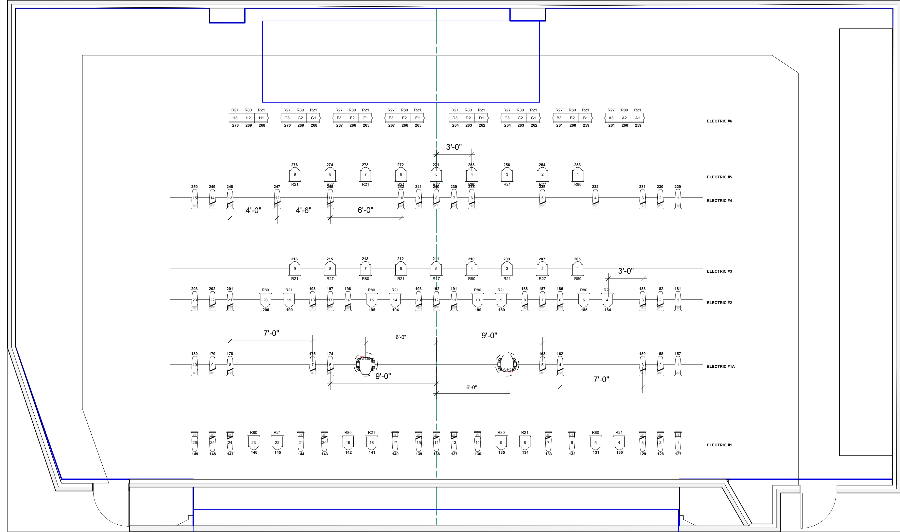
Mimi OHIO THEATRE LIGHT PLOT Scale: 1/4" = 1'-0"
